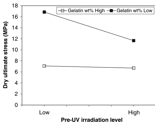
Fig. 5 Interaction effect between pre-UV irradiation time (factor 1) and gelatin wt% (factor 2). Pre-UV irradiation time is observed to have a larger effect at lower gelatin wt%
