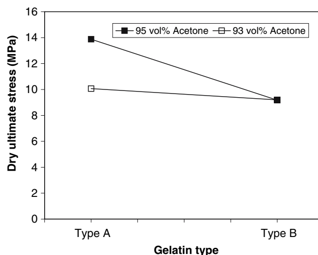
Fig. 6 Interaction effect between gelatin type (factor 5) and acetone vol% (factor 6). Gelatin type is observed to have a larger effect at higher acetone vol%
