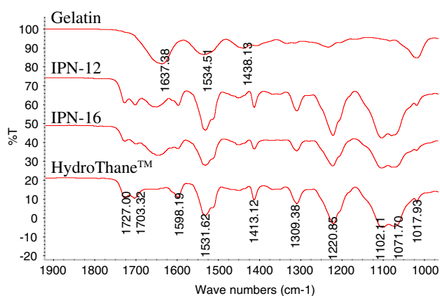
Fig. 2 FTIR spectra of gelatin, HydroThane™ and gelatin–HydroThane™ IPN fibers. The IPN fibers were prepared from experimental conditions #12 and #16 in Table 1. Spectra clearly show IPN to be a gelatin–HydroThane™ composite with tunable composition
